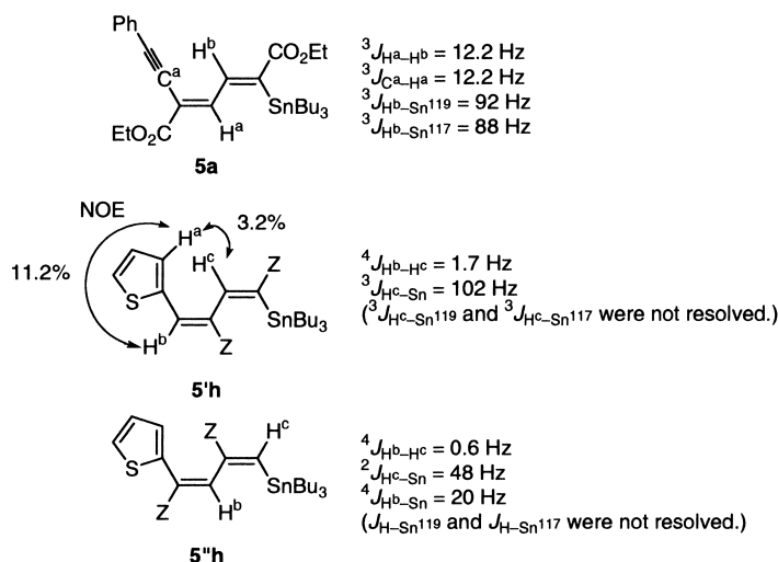
Fig. 1. Structure determination of dimerization–carbostannylation products.
