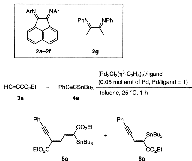
Scheme 2. Reaction of 3a with 4a in the presence of Pd-2 complexes.
