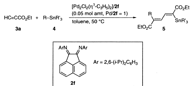
Scheme 5. Pd- 2f -catalyzed dimerization–carbostannylation.
