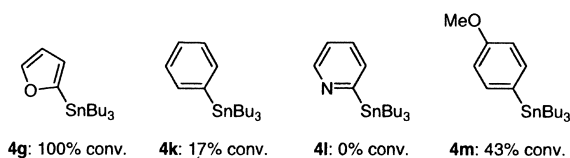
Scheme 4. Dimerization–carbostannylation of arylstannanes.
