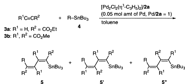
Scheme 3. Dimerization–carbostannylation of alkynes catalyzed by Pd-2a.
