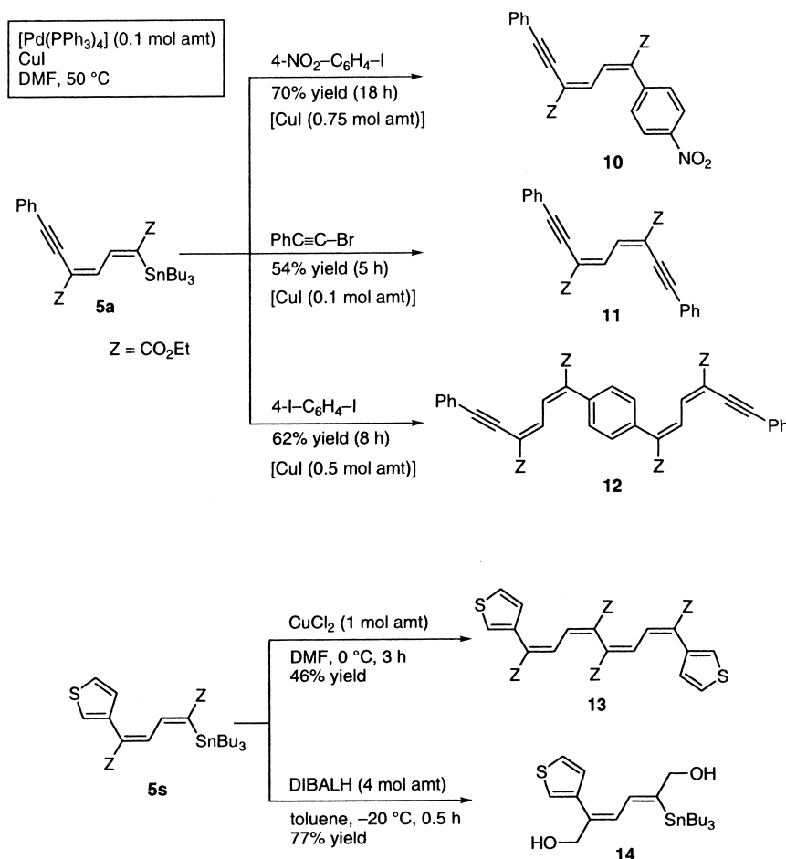
Scheme 8. Transformation of dimerization-carbostannylation products.
