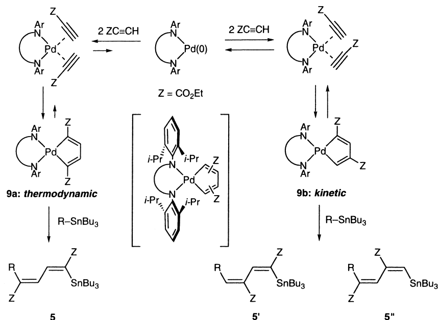
Scheme 7. Plausible catalytic cycle of the dimerization–carbostannylation.
