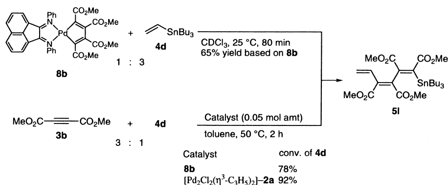
Scheme 6. Reactions using palladacycle 8b .
