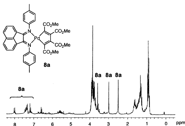
Fig. 2. ^1\text{H} NMR (200 MHz) spectrum of the reaction mixture (at ca. 31% conversion) in the reaction of 3b with 4d in the presence of [\text{Pd}_2\text{Cl}_2(\eta^3\text{-C}_3\text{H}_5)_2]\text{-2e} complex (0.2 mol amt of Pd, Pd/ 2e = 1) in \text{CDCl}_3 at 25^\circ\text{C} .
