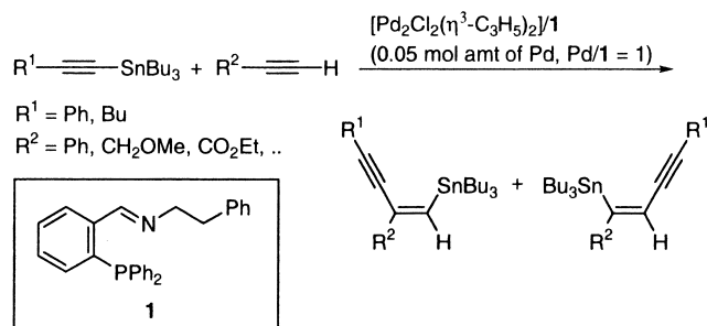
Scheme 1. Pd-iminophosphine-catalyzed alkenylstannylation of alkynes.
